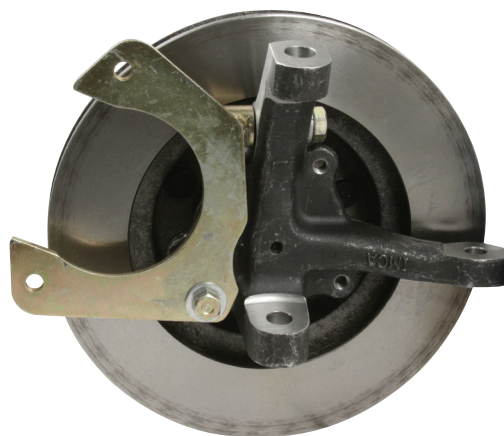
LH Spindle Shown With ALL42110 Bracket (Brackets Available In Black Only, Gold Shown For Illustration Purposes)
