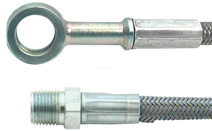
ALL46441-(Length) 1/8" Male NPT and 10mm Banjo Ends
