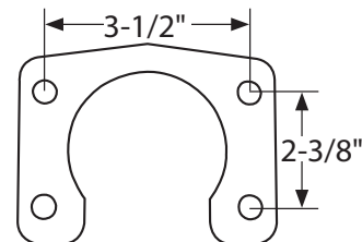
ALL72317 Large Bearing Early Style With 1/2" Hardware
